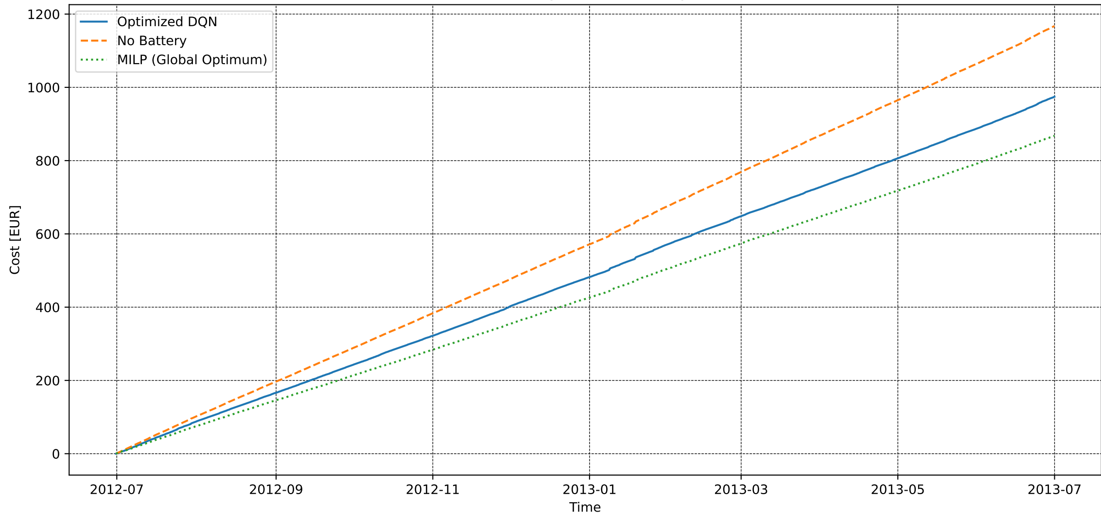
User 204 - Extended Convergence - Electricity Cost [DQN vs MILP]
